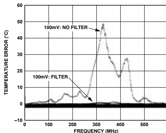
Figure 3. Effect of Filter on 100 mV Noise
