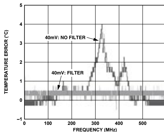
Figure 2. Effect of Filter on 40 mV Noise
